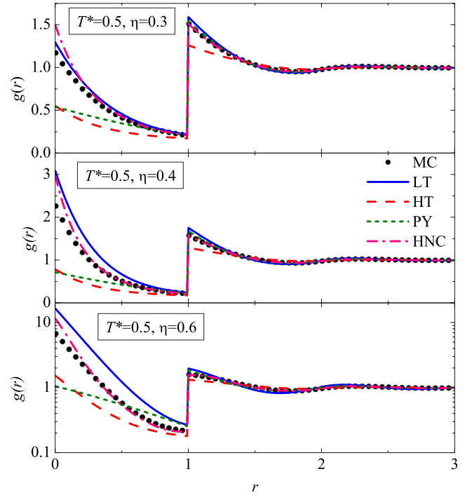
FIG. 4. (Color online) Plot of the radial distribution function at T^*=0.5 and for densities \eta=0.3 , \eta=0.4 , and \eta=0.6 . The circles are MC simulation data, while the lines correspond to the LT approximation (—), the HT approximation (---), the PY theory (· · ·), and the HNC theory (-·-·).
