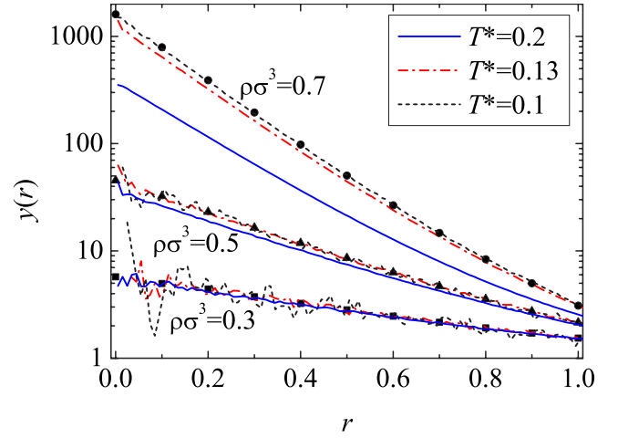
FIG. 1. (Color online) Plot of the cavity function y(r) inside the core ( r < 1 ) for densities \rho\sigma^3 = 0.3 , \rho\sigma^3 = 0.5 , and \rho\sigma^3 = 0.7 . The symbols are MC simulation data for HSs [31]. The lines are our MC data for PSs at T^* = 0.2 (solid lines), T^* = 0.13 (dashed-dotted lines), and T^* = 0.1 (dashed lines).
